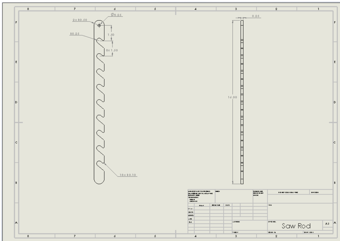
Figure C.3: Saw tooth Drawing
