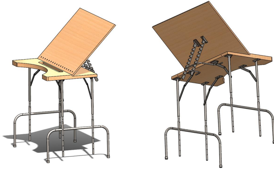
Figure 3: Left – Easel front view. Right – Easel back and below view
