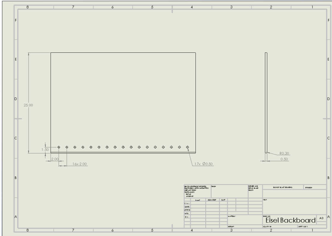
Figure C.2: Eisel Backboard Drawing
