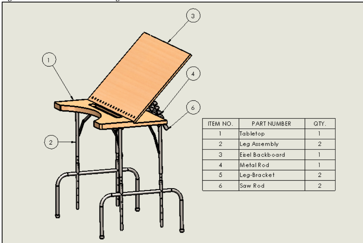
Figure 4: Complete Easel Design with labeled sublevel system parts (leg bracket not shown)
